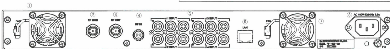
①FAN左 ②RF MON ③RF OUT ④RF IN ⑤VIDEO IN AUDIO IN L/R ⑥LAN ⑦FAN右 ⑧AC IN
